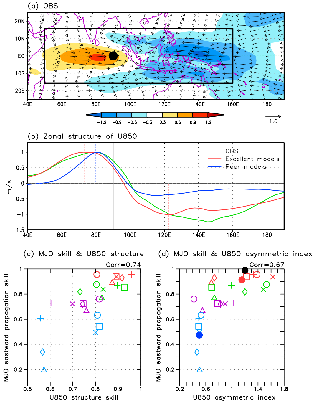
FIG. 4. Zonal asymmetry in the low-level circulation. (a) Observed structures of 850-hPa winds ( m s^{-1} ; vector) and zonal wind speed (U850) ( m s^{-1} ; shading). (b) Comparison of the longitudinal variations of the U850 in the observations, the composite of the excellent models, and the composite of the poor models. (c) The relationship between MJO eastward propagation skill and the PCC skill for U850 structure. (d) As in (c), but for the U850 asymmetric index, which is defined as the ratio of the maximum Kelvin easterly speed vs the maximum Rossby westerly speed, both of which are averaged between 5^{\circ}S and 5^{\circ}N . The black filled circle represents the observations. The structures in (a) and (b) are reconstructed using the same methods as is used in Figs. 2a and 2b, respectively. The regressed fields in (b) are normalized by their maximum values. The skill levels in (c) and (d) are computed using the same method as used in Fig. 2c.
