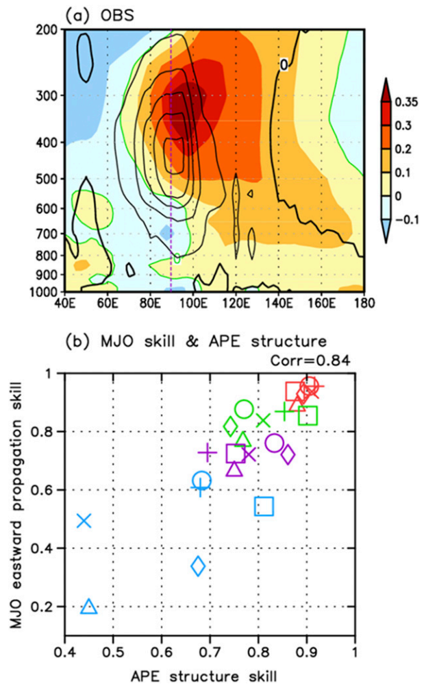
FIG. 8. (a) Eddy APE generation rate ( K^2 \text{ day}^{-1} ; contour) and temperature anomalies (K; shading) averaged between 5°S and 5°N. (b) The relationship between MJO propagation skill and PCC skill for the vertical structure of APE. The structures in (a) and the skill levels in (b) are computed using the same methods as are used in Fig. 5a and Fig. 2c, respectively.
