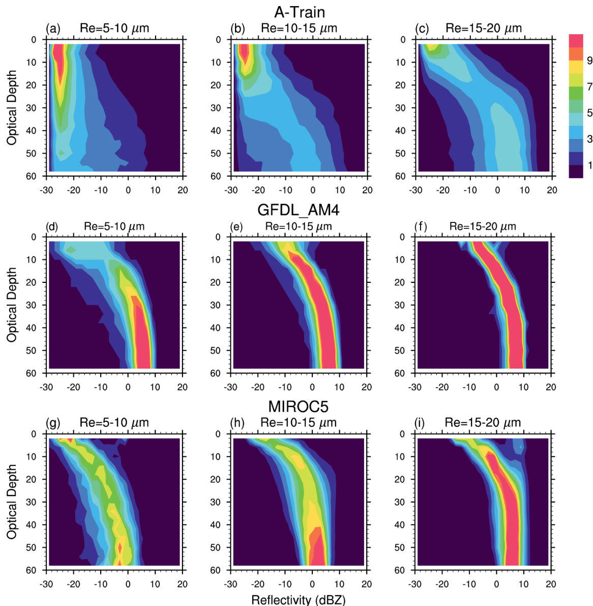
FIG. 6. The PDF (color shading; % dBZ -1 ) of radar reflectivity (abscissa) normalized as a function of cloud optical depth increasing downward (ordinate), which is further classified according to different ranges of cloud-top particle sizes for (left) 5–10, (center) 10–15, and (right) 15–20 \mu\text{m} obtained from (a)–(c) A-Train satellite observations, (d)–(f) GFDL AM4, and (g)–(i) Model for Interdisciplinary Research on Climate, version 5 (MIROC5; adapted from Jing et al. 2017).
