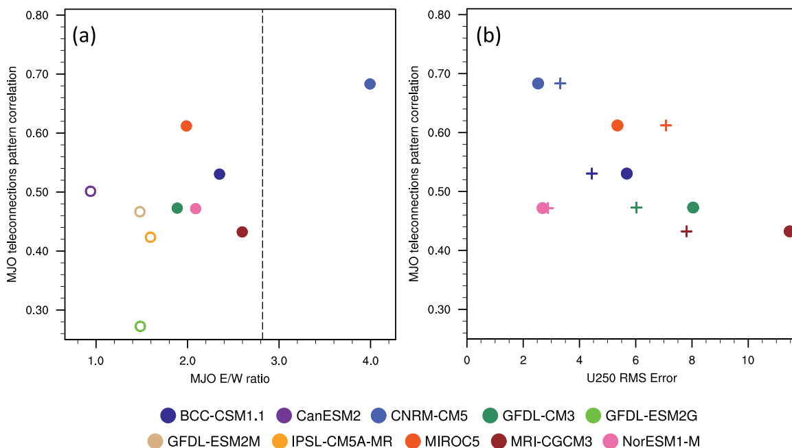
FIG. 2. From Henderson et al. (2017). December–February teleconnection performance averaged across all MJO phases (y axis) vs (a) MJO skill (MJO E/W ratio) and (b) the RMS error of the 250-hPa December–February zonal wind. The observed East/West (E/W) precipitation (GPCP) ratio is provided (dashed line, left panel). The MJO skill is derived as the ratio of eastward to westward power of equatorial precipitation in the 30–60-day, zonal wavenumber-1–3 band (e.g., Ahn et al. 2017). Teleconnection performance was determined as pattern correlation of North Pacific and North America (15°S–80°N, 130°E–60°W) MJO composite 250-hPa geopotential height anomalies between CMIP models and ERA-Interim averaged over all MJO phases. In (b), the crosses show the model 250-hPa zonal wind RMS error over the full Pacific basin, while the closed circles indicate the longitudinal RMS error of the subtropical jet. See the text and Henderson et al. (2017) for more detailed explanations.
