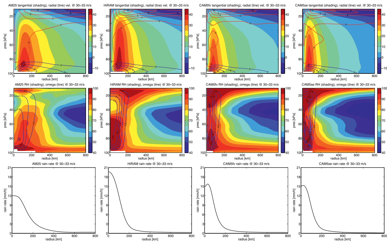
FIG. 7. (top),(middle) Azimuthally averaged radius–pressure plots of (top) tangential velocity (shading) and radial velocity (lines) and (middle) relative humidity (shading) and pressure velocity (lines). (bottom) Azimuthally averaged rain rate. All panels show the composites when the simulated tropical cyclones have a similar intensity, in this case between 30 and 33 m s -1 . Positive (negative) values are plotted in red (blue) contour lines. Four different GCM simulations [GFDL AM2.5 and High Resolution Atmospheric Model (HiRAM) models at 0.5° resolution and NCAR Community Atmosphere Model version 5–Finite Volume (CAM5-FV) and CAM5-Spectral Element (CAM-SE) models at 0.25° resolution] are used.
